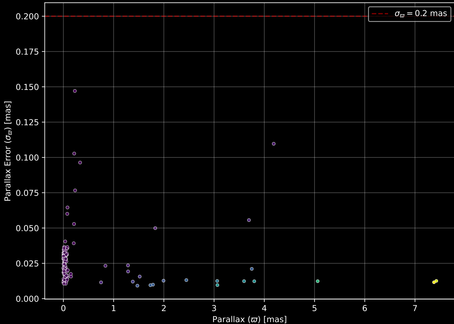
APOGEE DR17 Field: [LMC4] Parallax Quality (n= 154)
