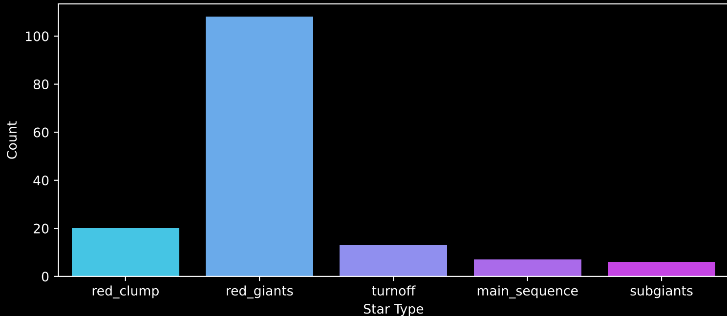
APOGEE DR17 Field: [LMC4] Count plot of Star Type
