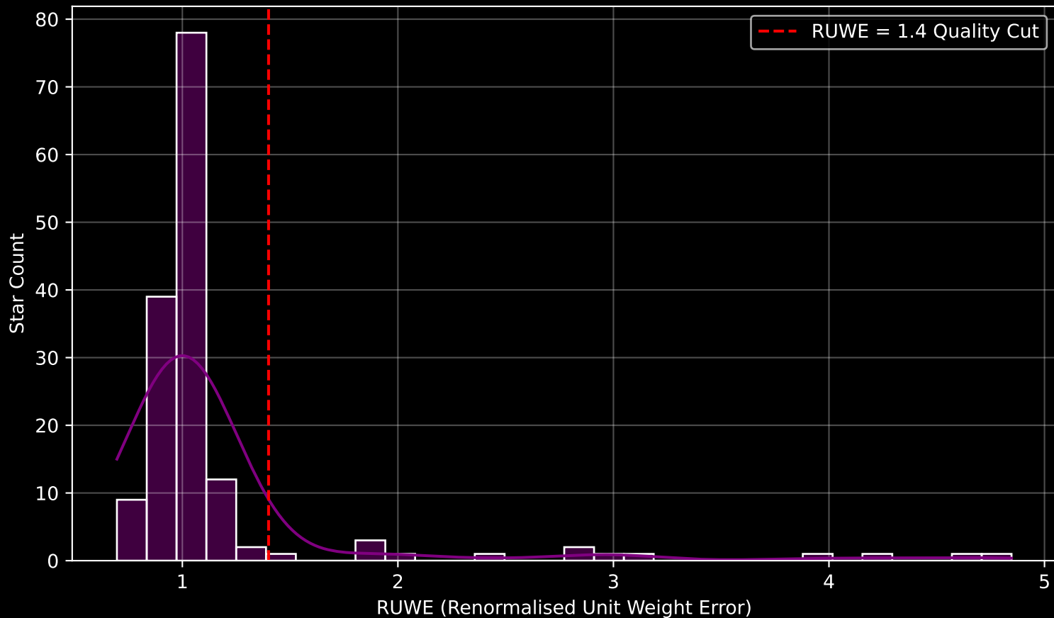
GAPOGEE DR17 Field [LMC4] RUWE Distribution (n= 154)
