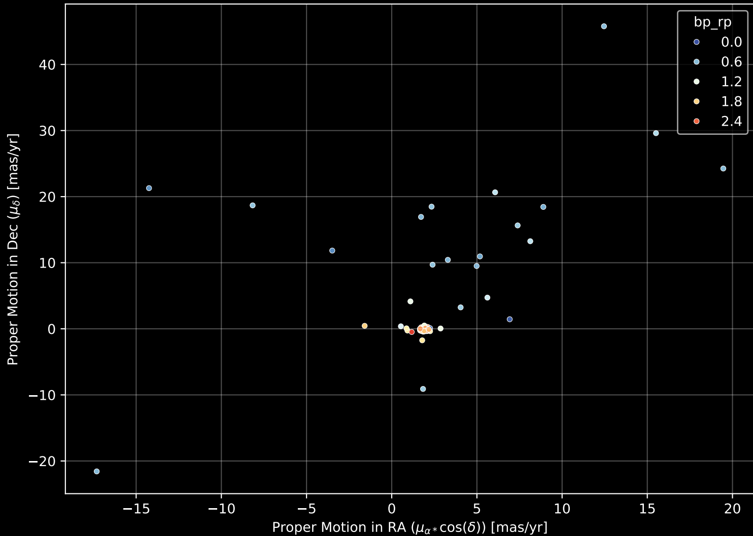
APOGEE DR17 Field: [LMC4] Proper Motion Diagram (n= 154)
