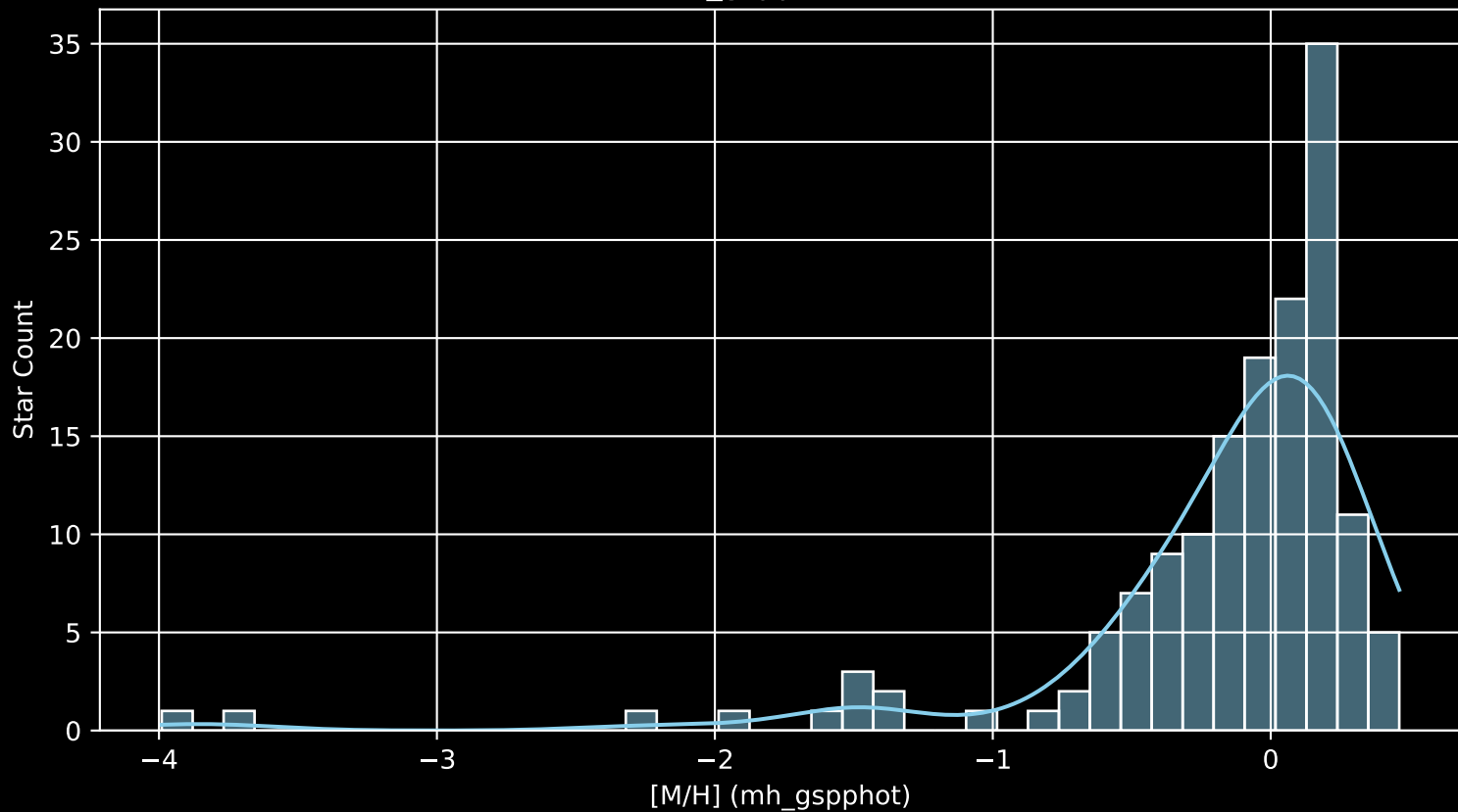
APOGEE DR17 Field: [LMC4 [M/H] (mh_gspphot) (n= 152)
