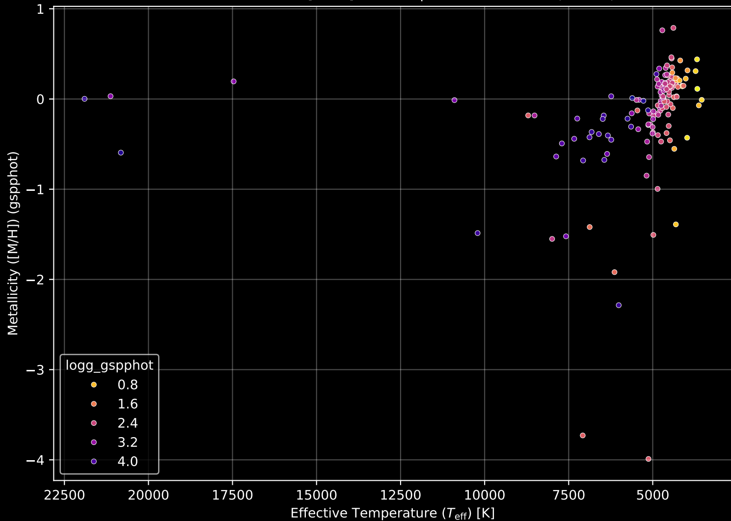
APOGEE DR17 Field: [LMC4] Stellar Population Parameters (n= 154)
